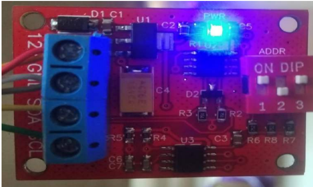
Pic. 7. Printed board of the temperature sensor module
