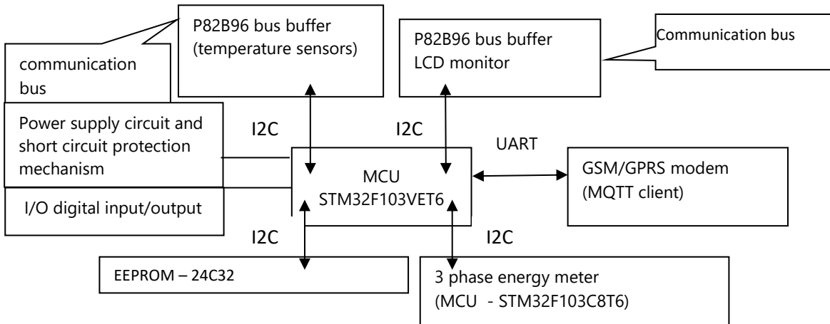
Pic. 2. Central controller block diagram
