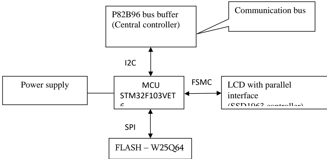
Pic. 4. LCD panel controller
