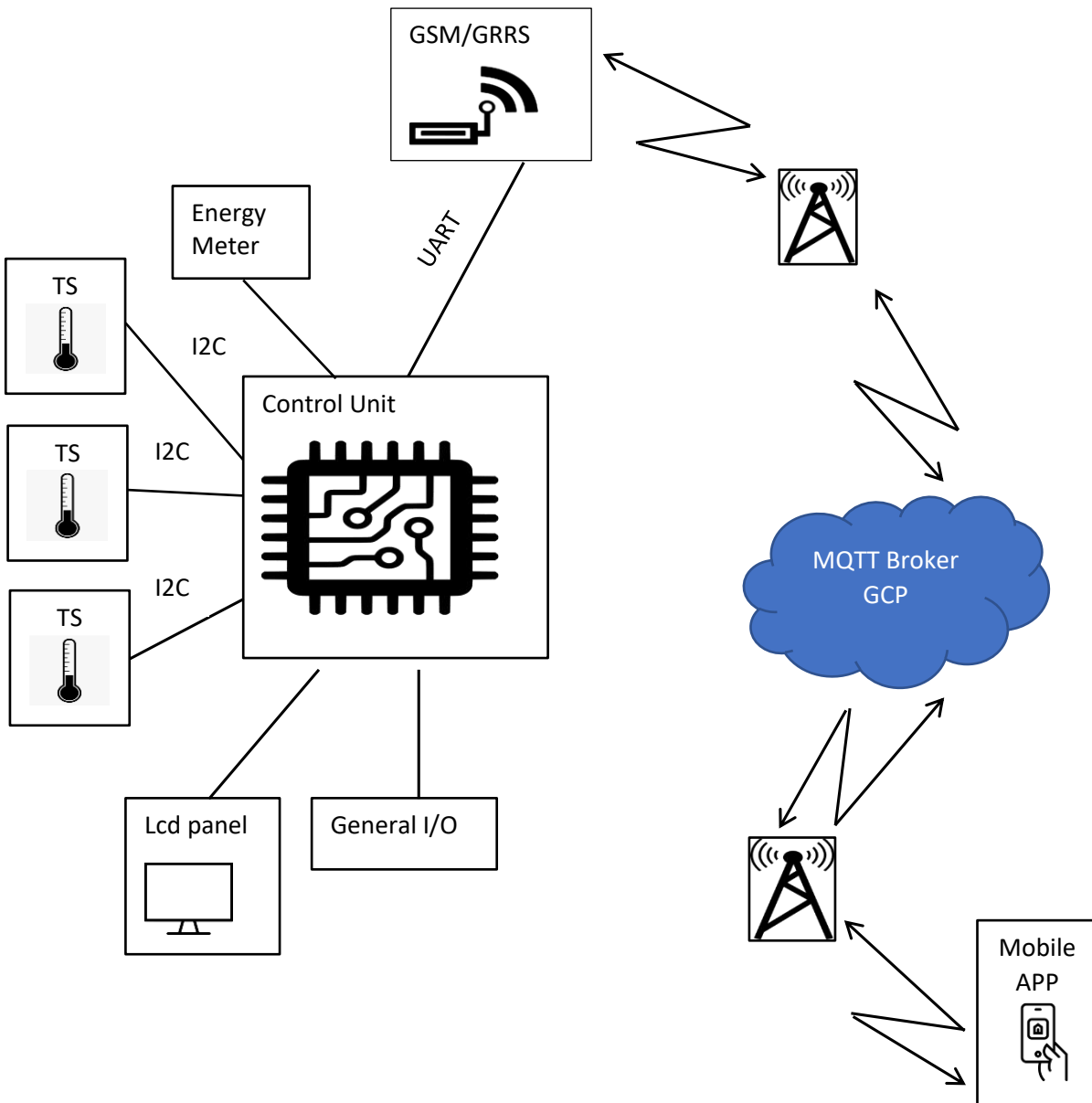
Pic. 1. Structure of IoT system of central heating
